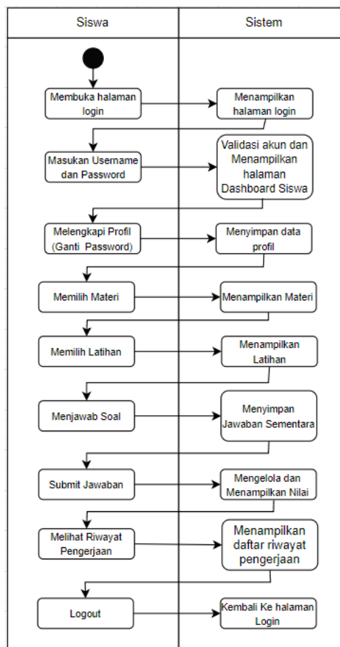
Gambar 1.3. 1 Activity Diagram
